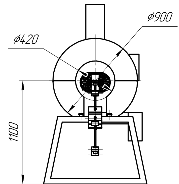
Conveyor oven for brake shoe bonding
